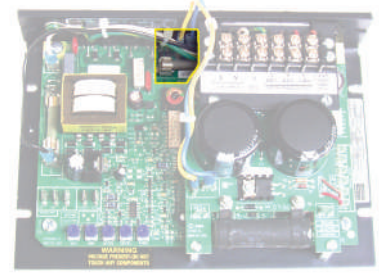
FIGURE 2. Location of motor fuse and quick connect tabs M+ and MF3.
