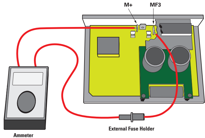
FIGURE 3. Connect ammeter and external fuse holder to M+ and MF3.
