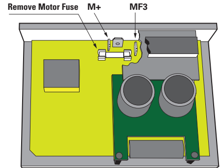
FIGURE 2. Location of motor fuse and quick connect tabs M+ and MF3.
